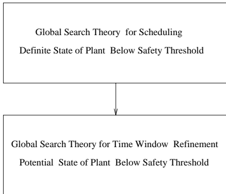
Figure 4. ROMAN's approach
